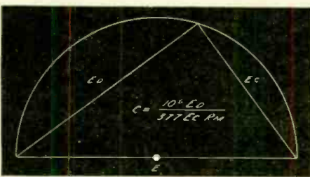
Fig. 9—Meters may be calibrated without recourse to cut-and-try, using the chart above.
